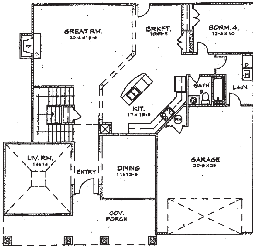
1ST LEVEL FLOOR PLAN
